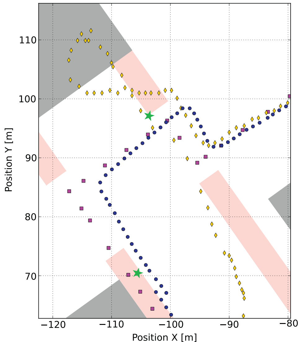
Fig. 5. Illustration of a real test realized in the Toulouse University campus. The squares indicate the travel that was really performed by the user. The diamonds indicate the positioning obtained with a commercial GPS. The dots indicate the positioning obtained with the NAVIG prototype. Visual Reference Points detected during the journey are indicated with stars.
