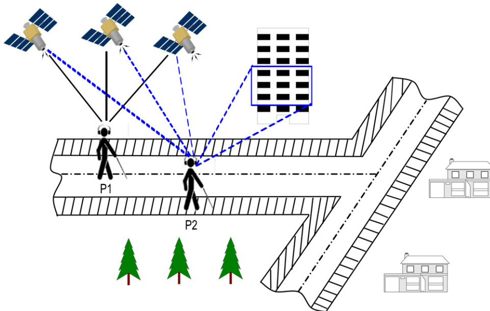
Fig. 3. Schematic principle of the regular (P1) and NAVIG (P2) positioning. User positioning P1 is the result of map matching GPS positioning with current commercial GIS. Using a Geographical Information System (GIS) including pedestrian areas and visual geolocated targets, the NAVIG positioning (P2) locates the user with a better precision, which is compatible with assisted navigation for the Blind.
